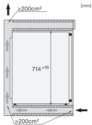
FNS7040E, FNS7040B, FNS7040C, FNS7040D, side view (installation drawings)
