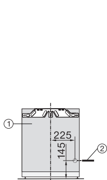
FNS7040E, FNS7040B, FNS7040C, FNS7040D, installation (*footnote) (installation drawings)
